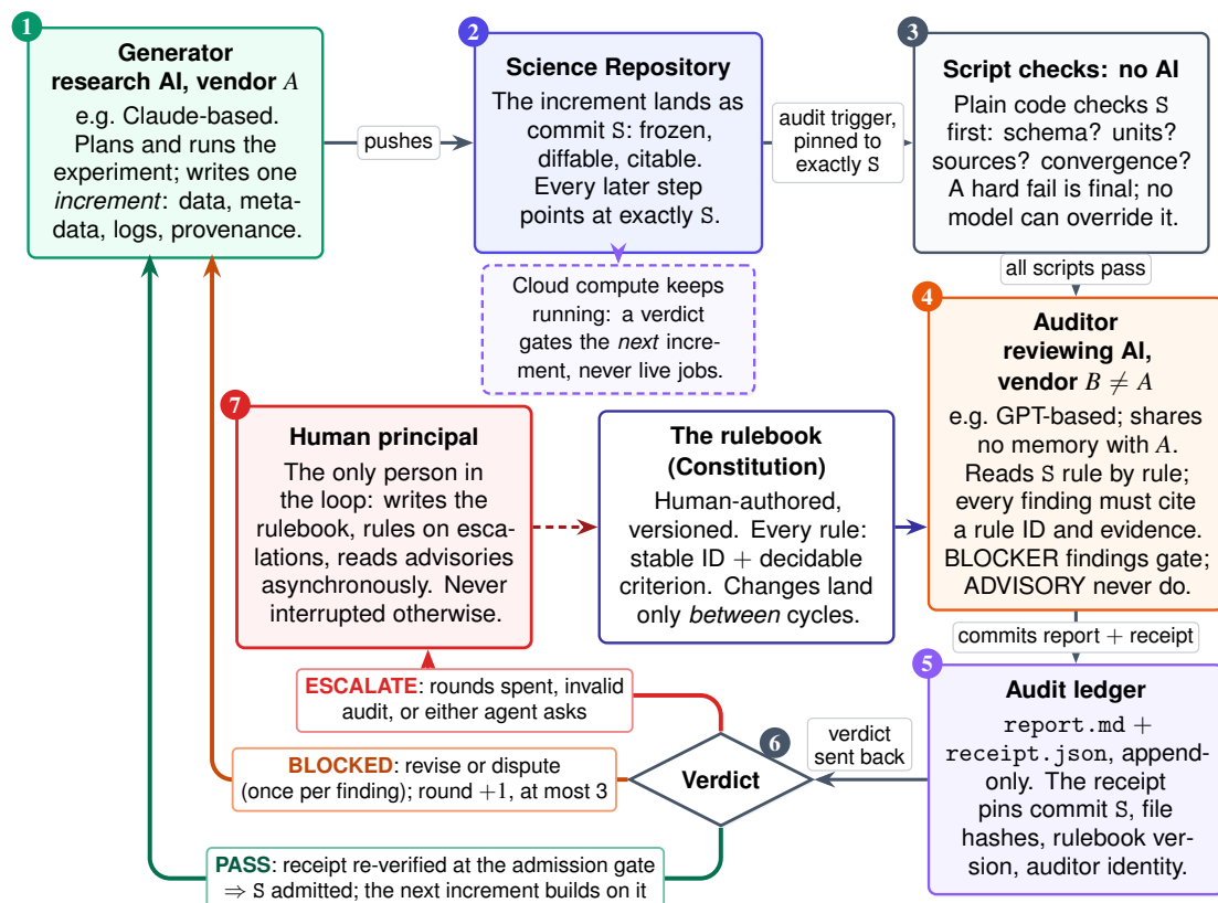
Figure 2: One experiment increment through the loop, read clockwise from the top left. Numbers give the order, and the three coloured paths out of the verdict are the only ways a cycle can end. Who may write where is Figure 1; the walk in full is §3.1 and §3.4.
