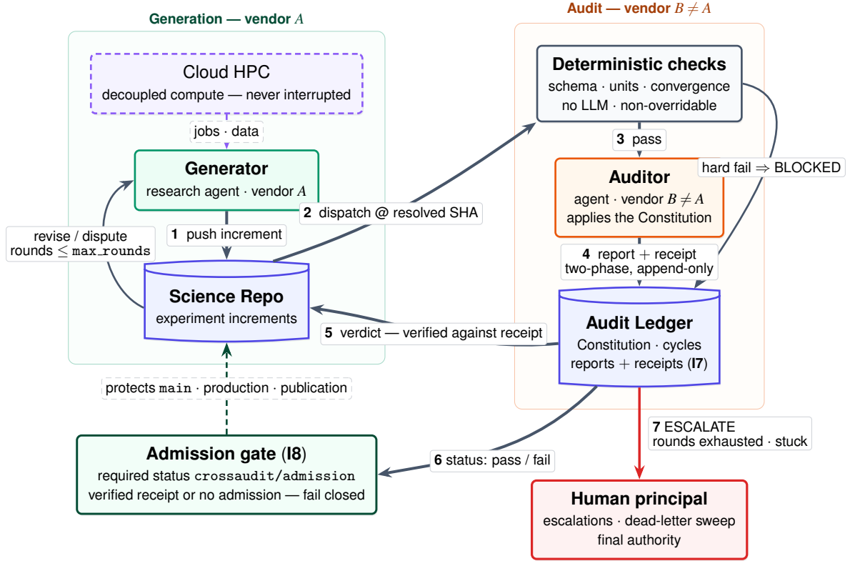
Figure 1: The CrossAudit loop, revision 1. Numbered arrows follow one increment: deterministic checks precede any model (I4); the audit side emits a two-phase report-plus-receipt into an append-only ledger (I7); the verdict is verified against the fetched receipt, and a required commit status gates protected actions fail-closed (I8); controller-managed rounds bound revision (I5); humans are interrupted only by escalation or the dead-letter sweep (I6).
