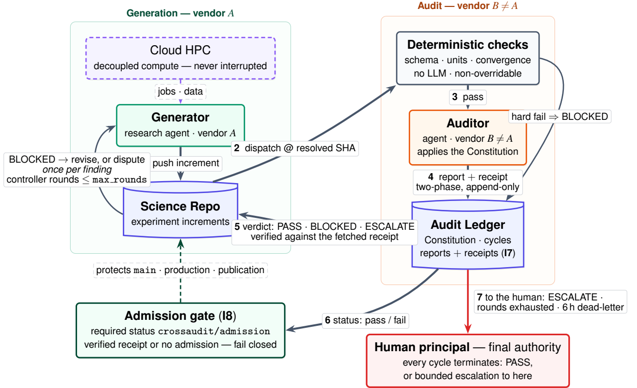
Figure 1: The CrossAudit loop, revision 1. Numbered arrows follow one increment: deterministic checks precede any model (I4); the audit side emits a two-phase report-plus-receipt into an append-only ledger (I7); the verdict is verified against the fetched receipt, and a required commit status gates protected actions fail-closed (I8); controller-managed rounds bound revision (I5); humans are interrupted only by escalation or the dead-letter sweep (I6). Termination is structural: within max_rounds every cycle ends in admission or in human hands, disputes are one-shot per finding, and silent stalls are caught by the sweep.
