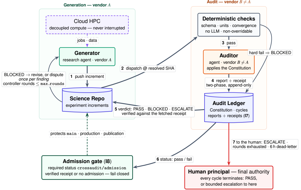
Figure 1: The CrossAudit loop, revision 1. Numbered arrows follow one increment: deterministic checks precede any model (I4); the audit side emits a two-phase report-plus-receipt into an append-only ledger (I7); the verdict is verified against the fetched receipt, and a required commit status gates protected actions fail-closed (I8); controller-managed rounds bound revision (I5); humans are interrupted only by escalation or the dead-letter sweep (I6). Termination is structural: within max_rounds every cycle ends in admission or in human hands, disputes are one-shot per finding, and silent stalls are caught by the sweep.
