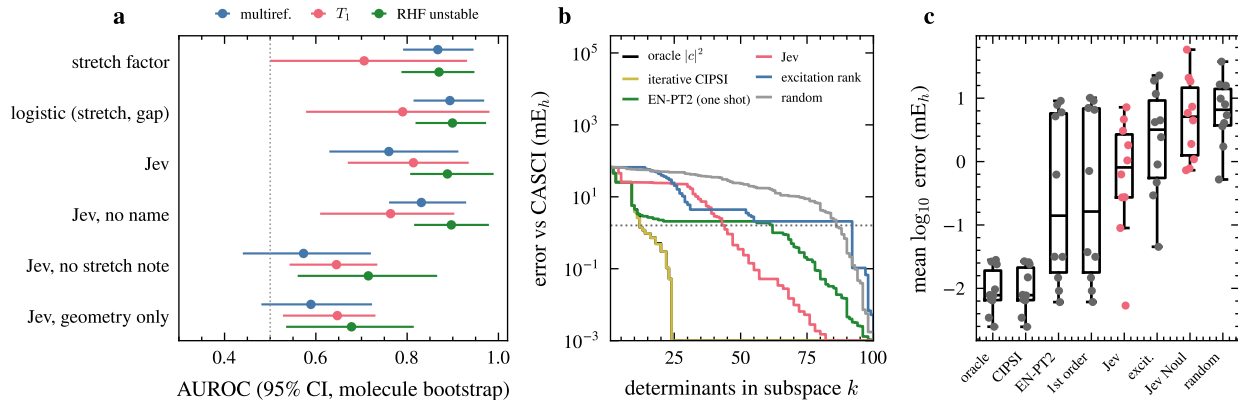
Figure 5: Jev in quantum-chemistry workflows. a , AUROC with 95% molecule-clustered bootstrap intervals for the three E3 labels, for the stretch factor alone, a logistic model, Jev, and three Jev input ablations. b , Selected-CI error against subspace size for N_2 at equilibrium, CAS(6e,5o)/cc-pVDZ; dotted line, 1.6 mE_h . c , Mean \log_{10} error over the whole curve for ten systems; lower is better. “Jev Noul” is the per-determinant elicitation.
