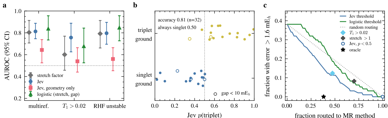
Figure 4: A larger set and a routing workflow (E5–E6). a , AUROC with molecule-clustered 95% intervals on 31 less common molecules for the stated stretch factor, Jev, Jev with geometry only, and a leave-one-molecule-out logistic model. b , Jev’s probability of a triplet ground state for 32 species, grouped by the CCSD(T) ground state; open markers have gaps below 10 mE h . c , Fraction of cases whose final error exceeds 1.6 mE h against the fraction routed to a multireference method, for thresholds on Jev and on the logistic model, the T_1 rule, a stretch rule, Jev’s own p < 0.5 threshold and an oracle.
