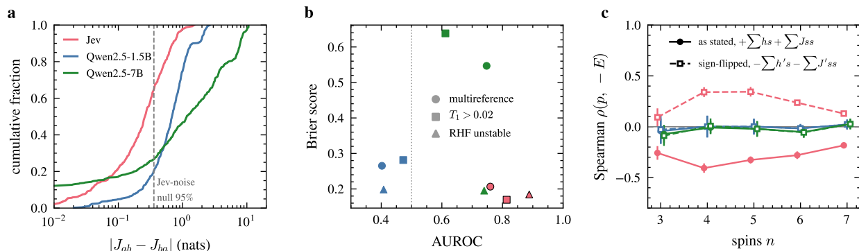
Figure 6: Jev against two open-weight models (E7). a , Cumulative distribution of coupling asymmetry over the 480 case-pair combinations of E1; the dashed line is the 95th percentile of a coherent null with Jev’s noise. b , AUROC and Brier score on the three E3 labels. c , Rank correlation between probability and negative energy for random Ising models written in both sign conventions; mean \pm s.e.m. over instances.
