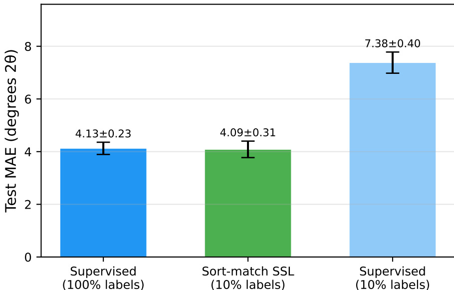
(a) Main Result: Sort-Match SSL Matches Full Supervision
