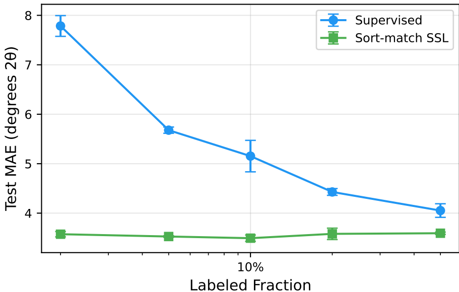
(b) SSL Advantage Grows at Low Label Fractions
