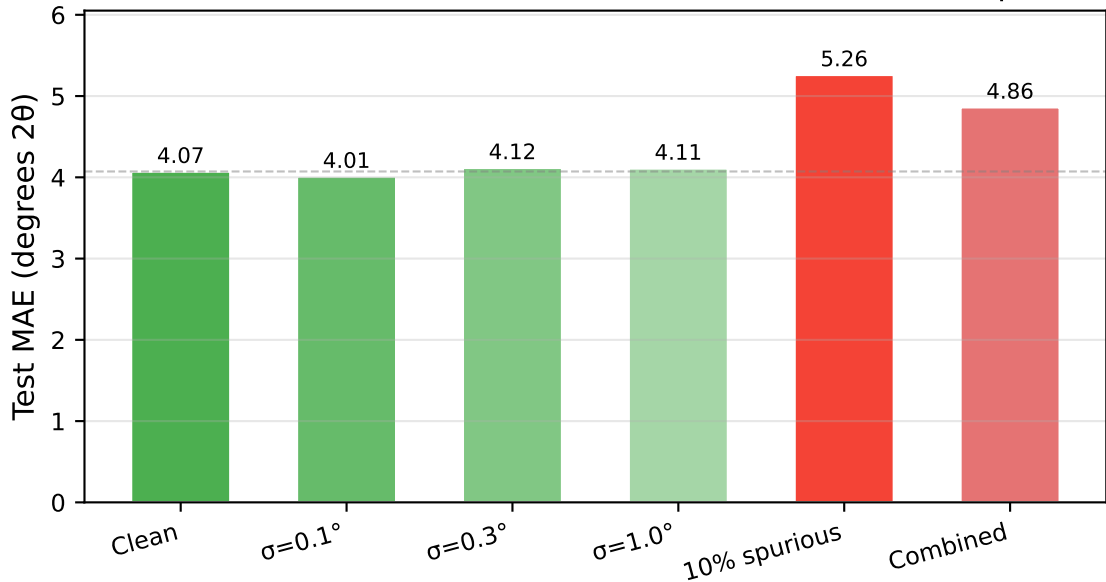
(c) Noise Robustness: Tolerant to Gaussian, Sensitive to Spurious
