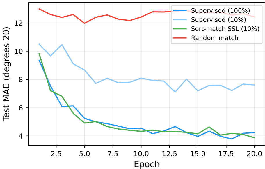
(e) Training Curves
