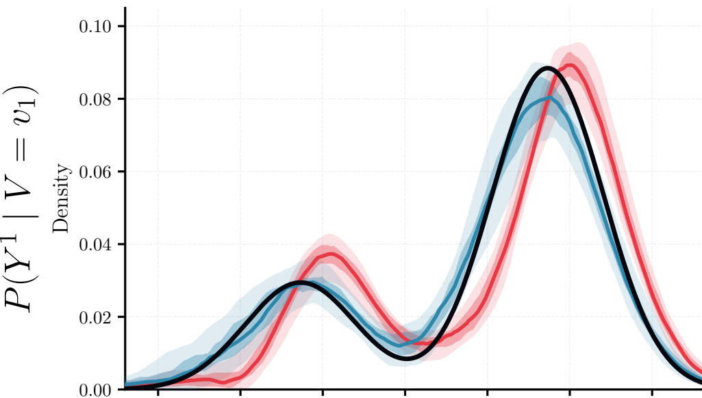
Ridge Regression
