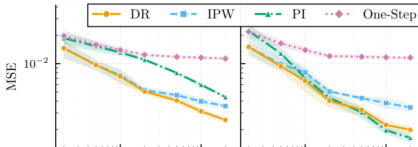
Ridge Regression
