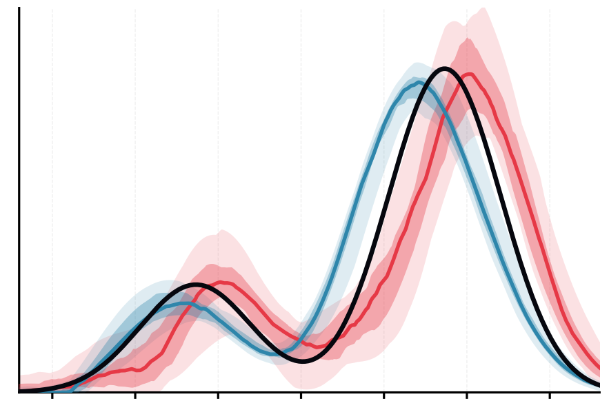
Neural-Kernel
