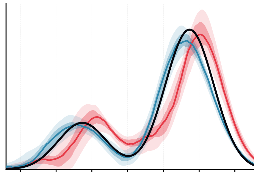
Deep Feature
