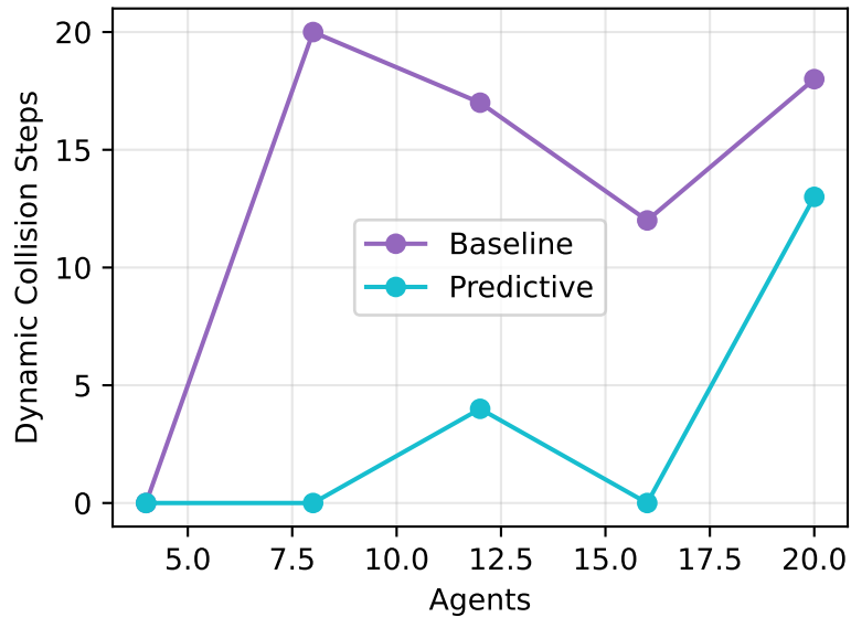
Dynamic Collision Steps
