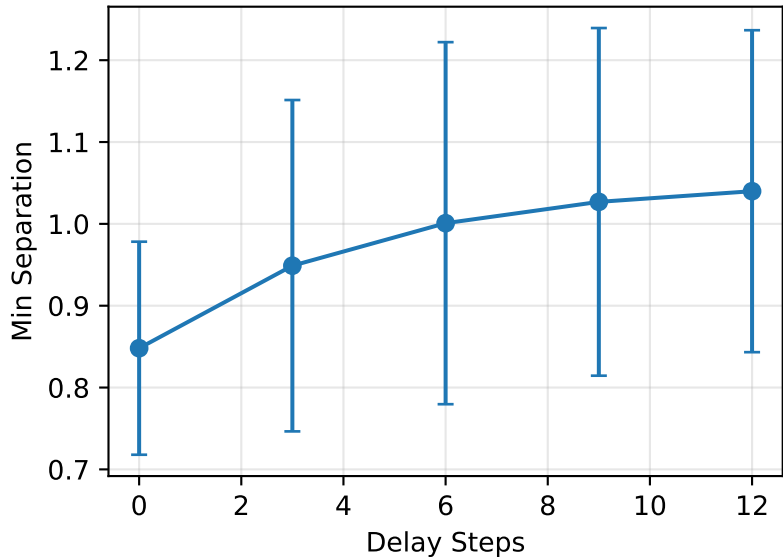
Min Separation
