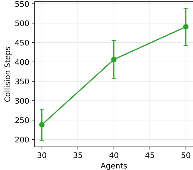
Collision Steps vs Agents
