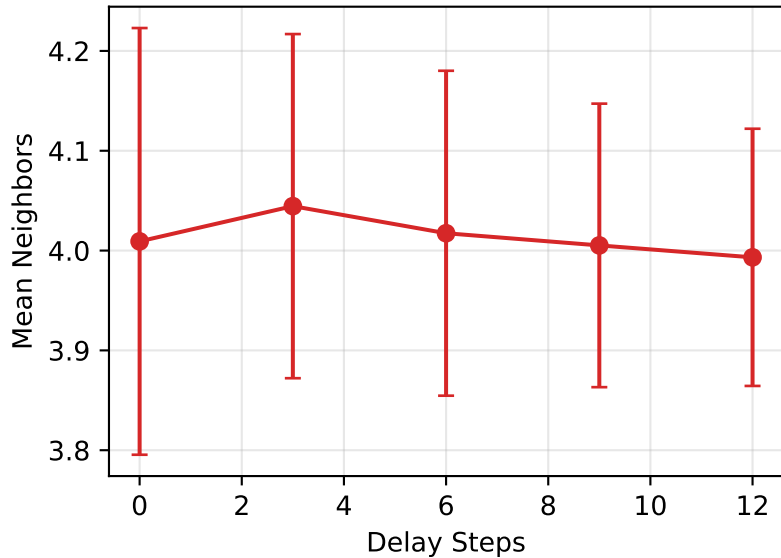
Mean Neighbors
