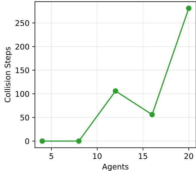
Collision Steps vs Agents
