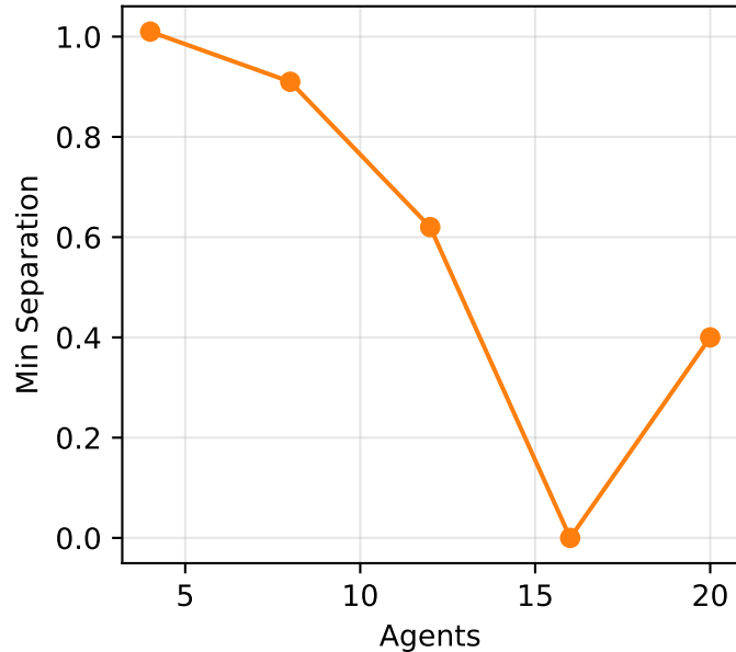
Min Separation vs Agents
