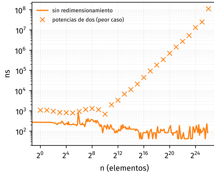
push
