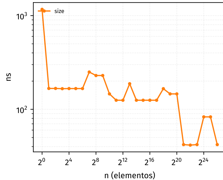
size
