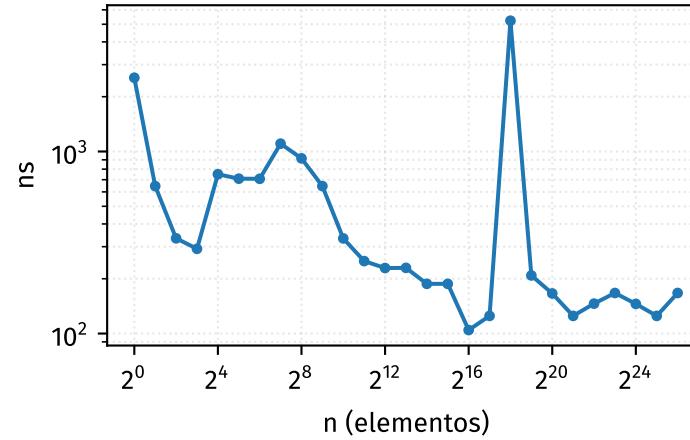
pushBack
