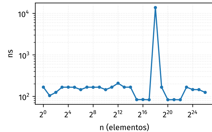
erase
