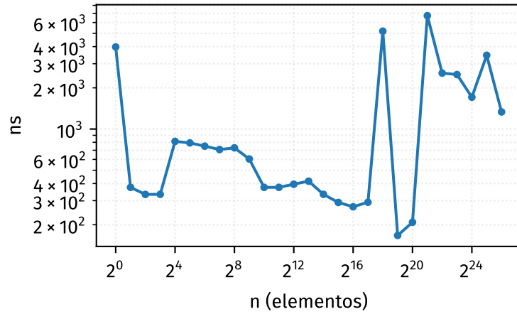
addBefore
