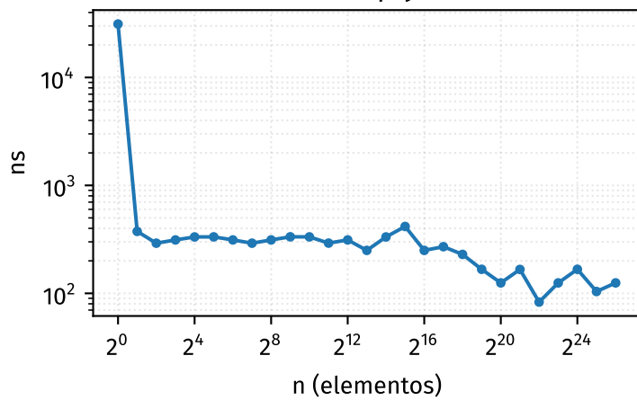
pushFront
