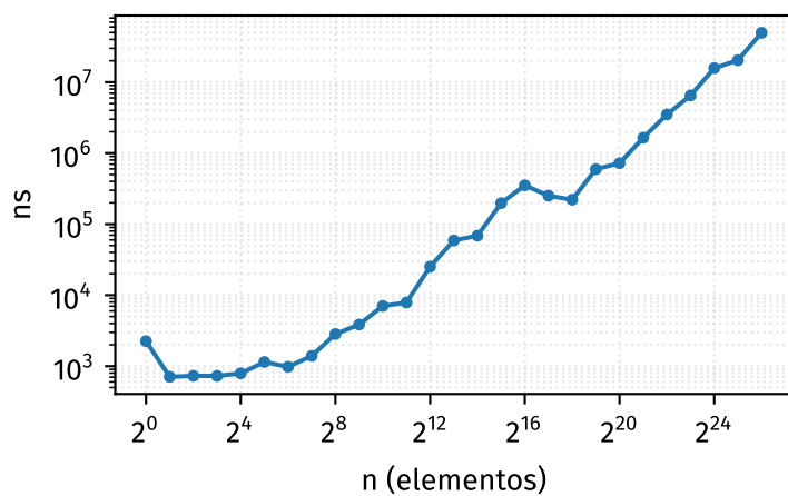
addBefore
