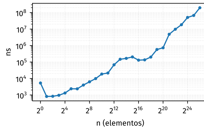
erase
