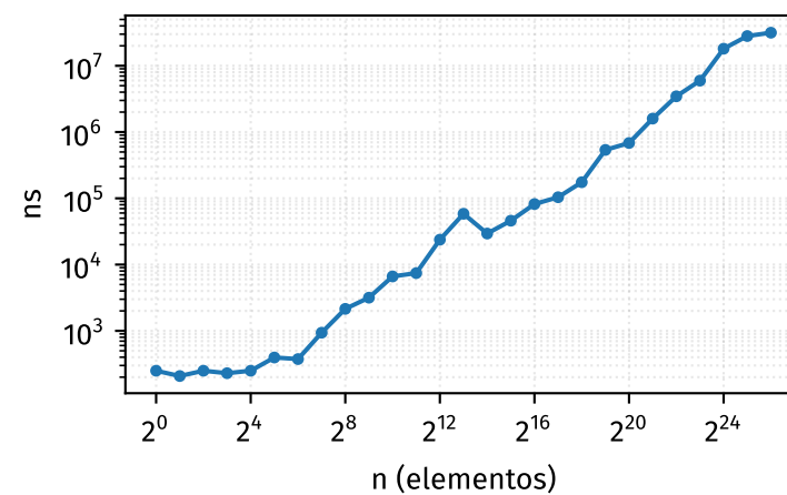
erase
