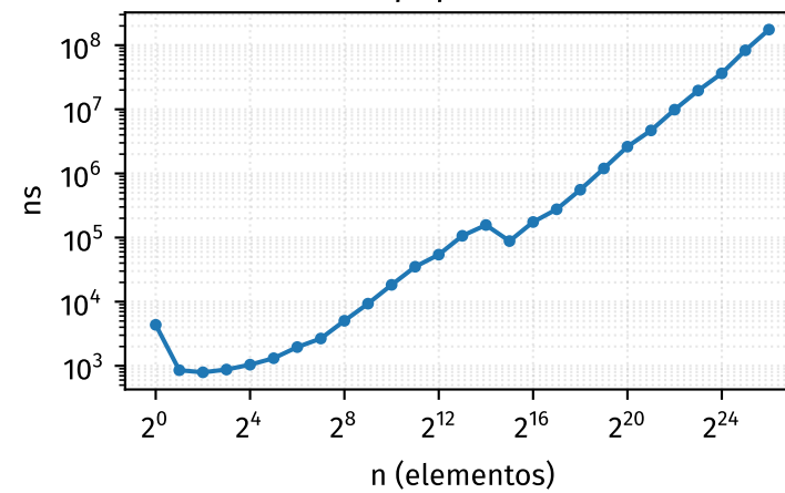
find
