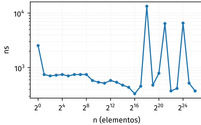
addBefore
