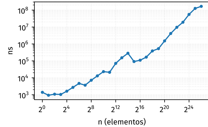
erase
