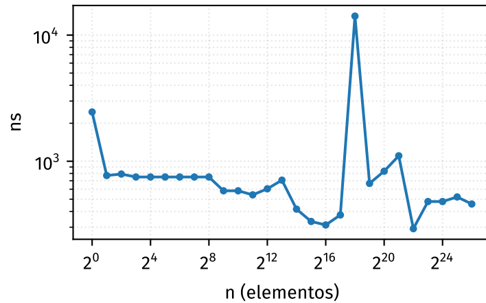
addBefore
