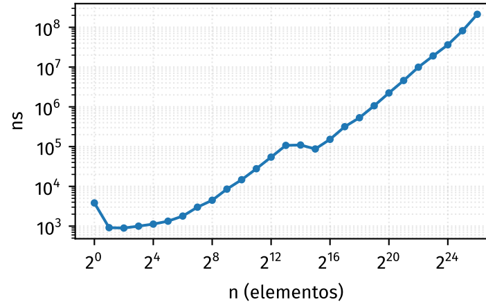
pushBack
