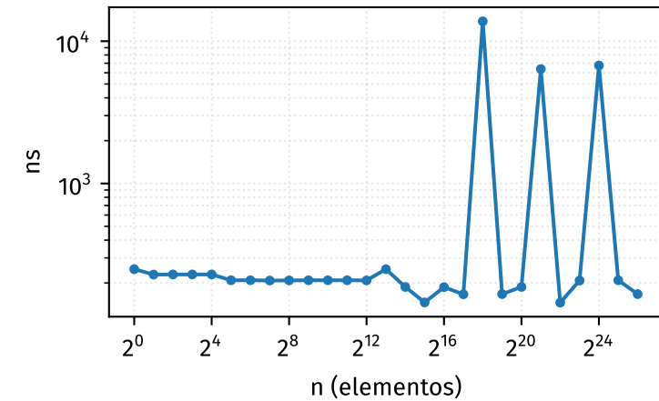
erase
