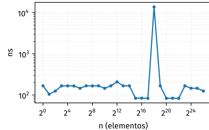
erase
