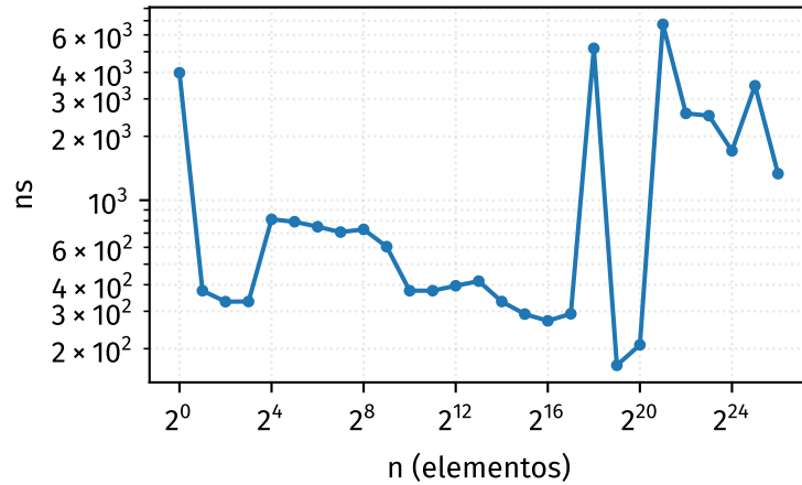
pushFront
