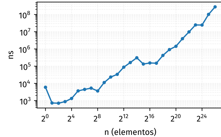
find
