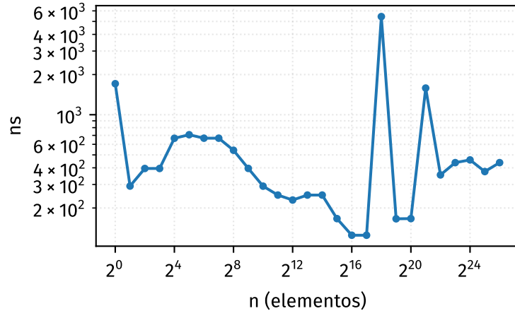
addBefore
