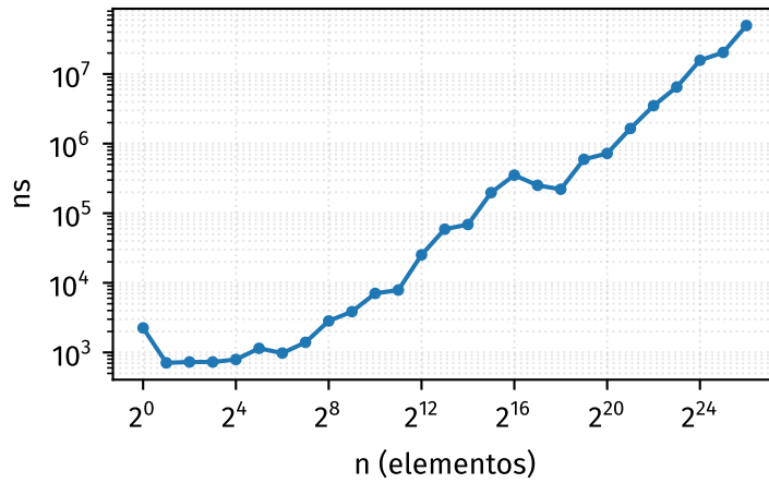
addBefore
