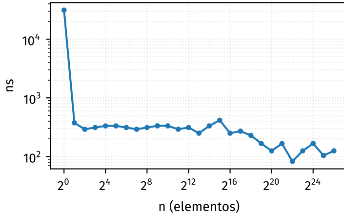
pushFront
