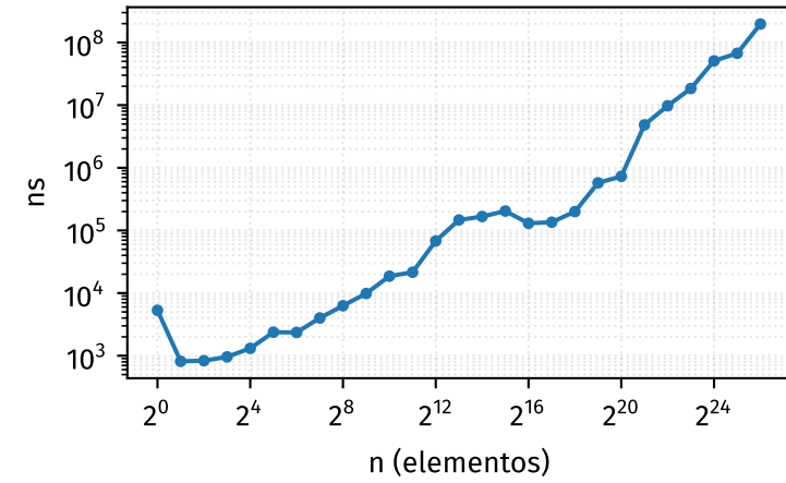
erase
