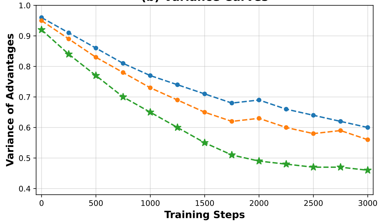
(b) Variance Curves
