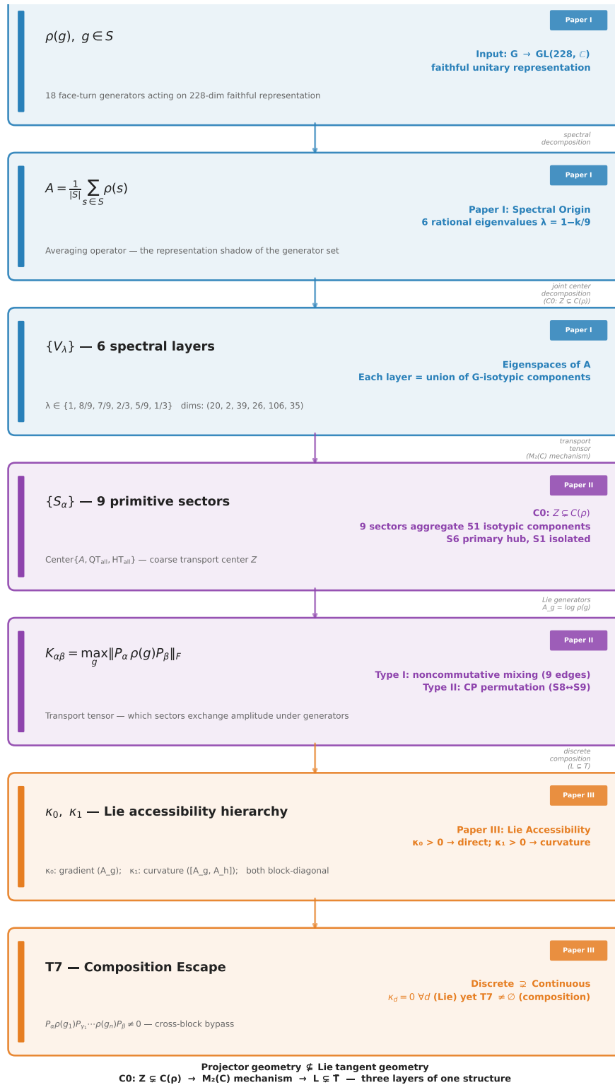
CCS Figure C0. Structural pipeline: trilogy weld — \rho(g) \rightarrow (QT\_all, HT\_all) \rightarrow \{S_\alpha\} \rightarrow A18 collision quotient \{V_\lambda\} \rightarrow K \rightarrow K_0/K_1 \rightarrow T7 .
