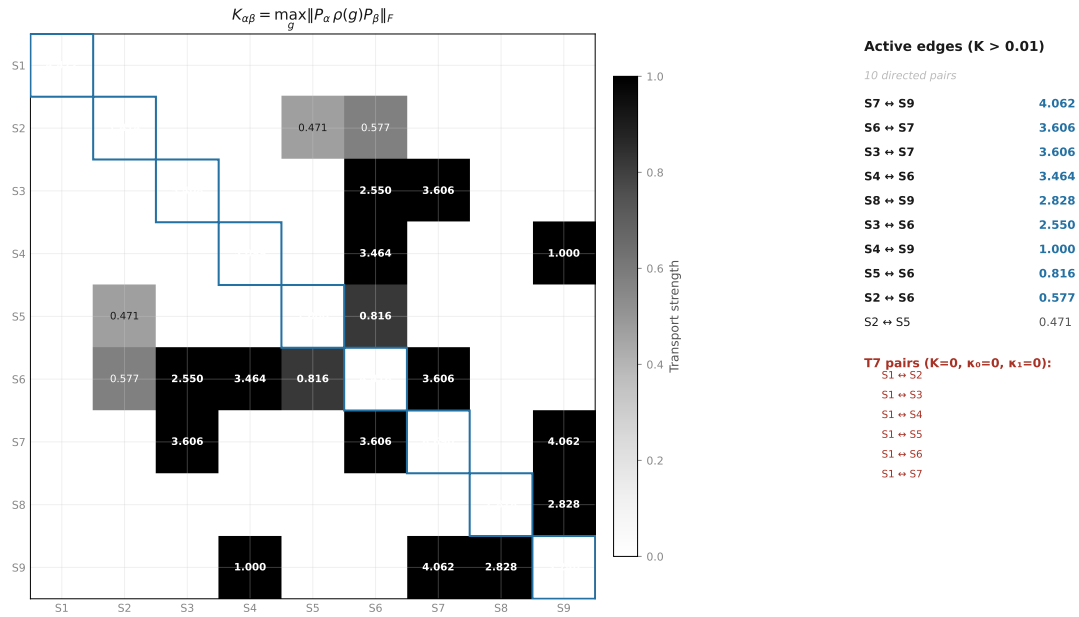
CCS Figure C2. Full 9 \times 9 transport matrix K_{\alpha\beta} heatmap with annotated values.
