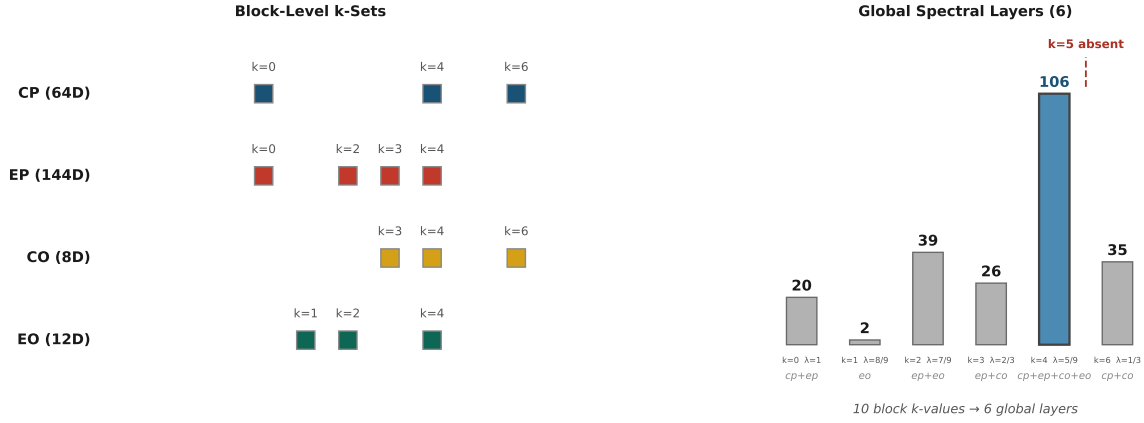
CCS Figure C9. Resonance merging: 10 block-level eigenvalues collapse to 6 global layers.
