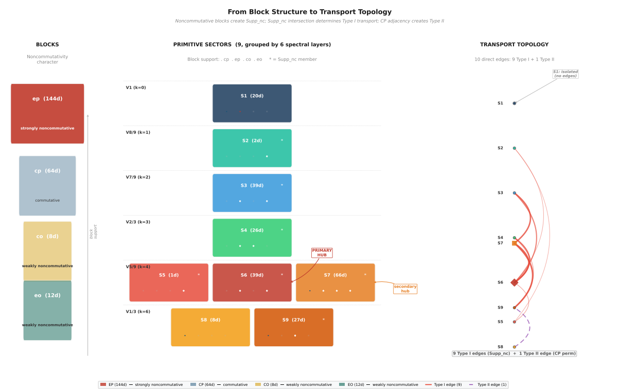
CCS Figure C17. Block-sector alluvial diagram: three-panel flow from 4 blocks (left, with qualitative noncommutativity labels) through 6 layers (center) to 9 sectors (right), tracing the algebraic origin of transport topology.
