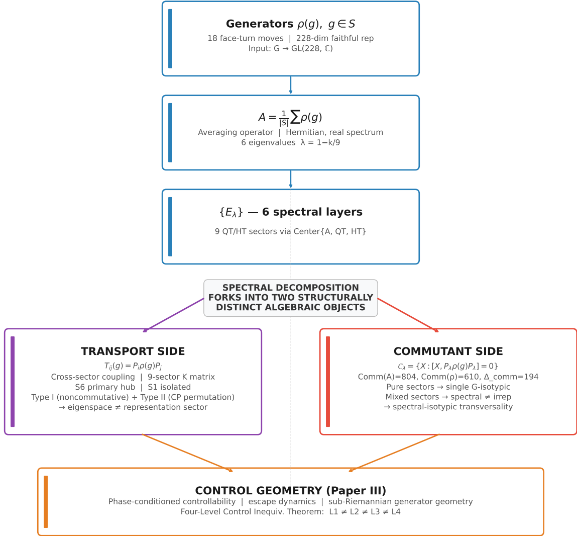
Figure 6. The structural pipeline from generators \rho(g) to the commuting QT/HT averages, their 9 joint-spectral sectors \{S_\alpha\} , and the A_{18} collision quotient \{E_\lambda\} . The resolved sector projectors define transport (left: K_{\alpha\beta} , Type I/II classification, T7 detection), while the same representation data define the commutant comparison (right: \text{Comm}(\rho) = 610 , \text{Comm}(A) = 804 , \Delta_{\text{comm}} = 194 ). The two branches are structurally independent in general but linked through the EP block's M_2 structure in this system.
