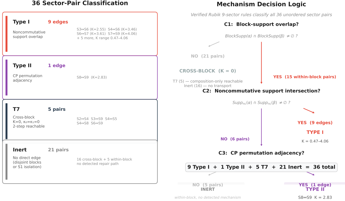
Figure 3. Transport mechanism classification for all 36 sector pairs: Type I (noncommutative overlap, 9 edges, K = 0.47 – 4.06 ), Type II (CP permutation adjacency, 1 edge, S8 \leftrightarrow S9 K = 2.83 ), T7 (cross-block composition-only, 5 pairs, K = 0 ), and Inert (21 pairs, no transport). Three criteria — block overlap, noncommutative support intersection, and CP adjacency — classify all 36 pairs without ambiguity. \text{Supp}_{\text{nc}} intersection is the verified criterion for Type I transport across the Rubik 9-sector system.
