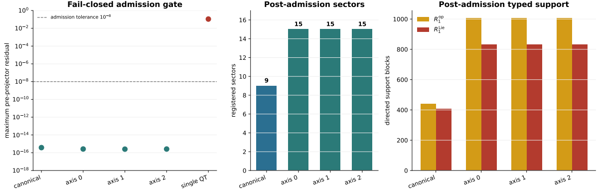
Figure 2. Normality-gated pointwise registrations. Five candidate samples enter the pre-projector gate. The single-QT control is rejected, while the canonical point and three QT-axis samples are admitted. Sector and typed direct-support counts are displayed only for admitted records. The figure supplies neither projector continuation nor a path theorem.
