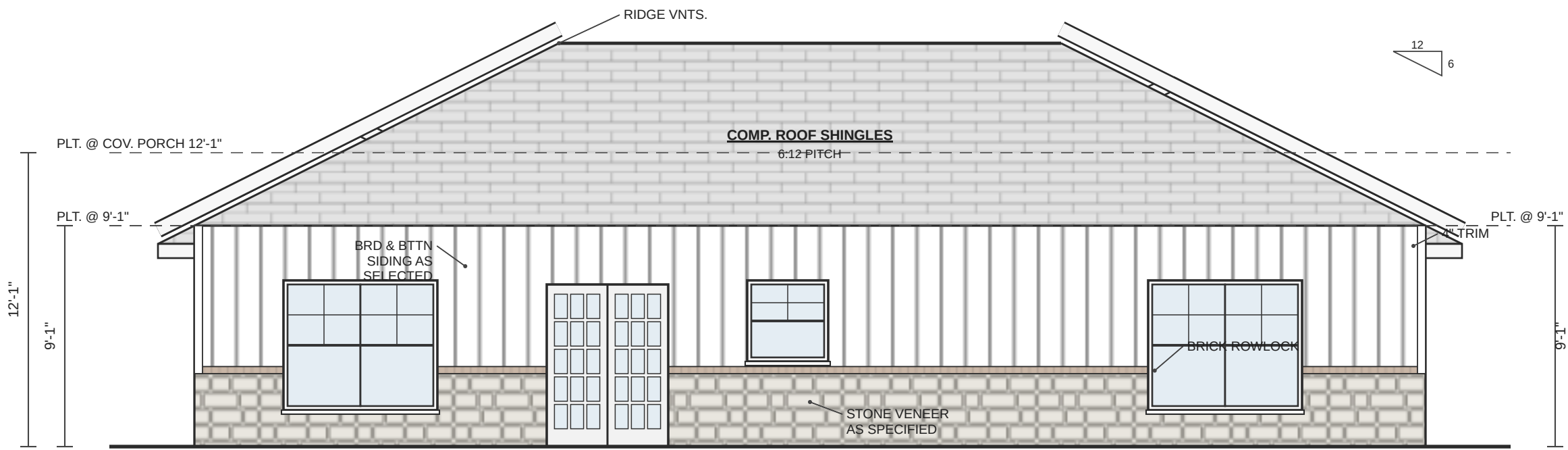
REAR ELEVATION SCALE: 3/16" = 1'-0"
