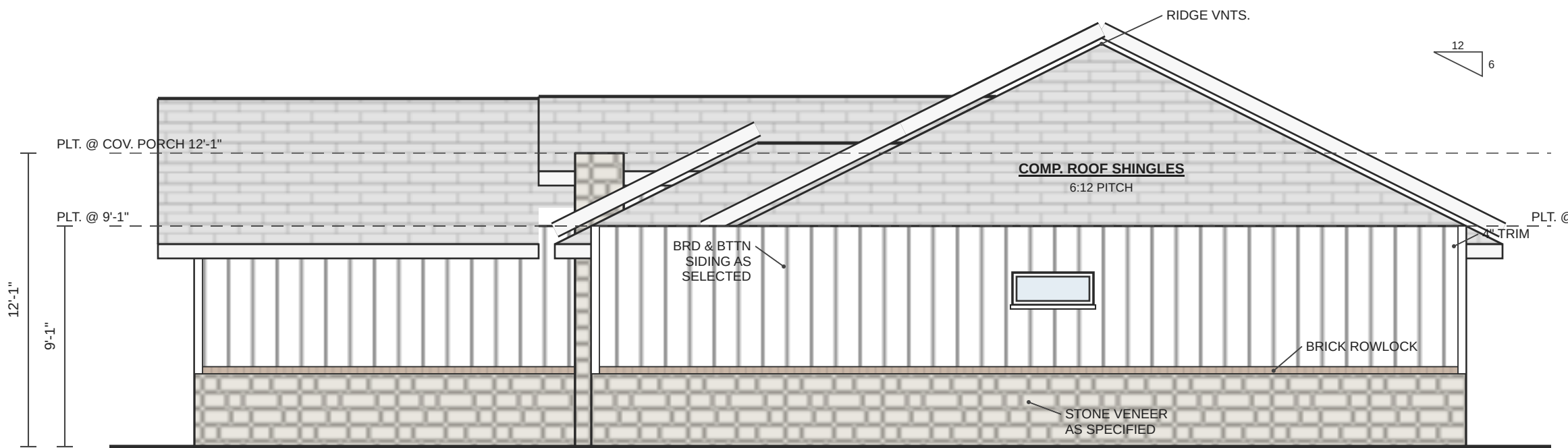
RIGHT ELEVATION SCALE: 3/16" = 1'-0"
