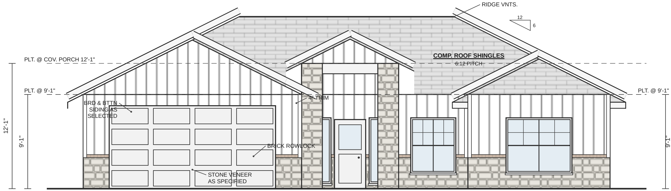
FRONT ELEVATION SCALE: 3/16" = 1'-0"
