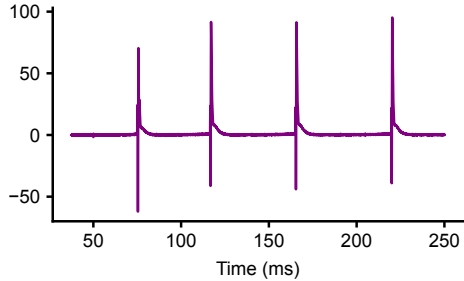
Optimal current with analytic computation
