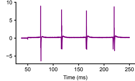
Optimal current for trained multi-compartment model
