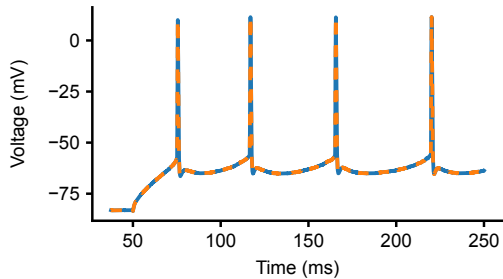
Root search - loss: 5.2472
