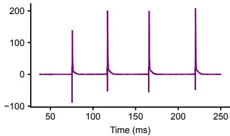
Optimal current with root search
