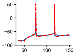
Loss: 115.3725
