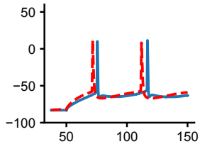
Loss: 116.8703
