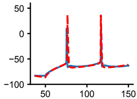
Loss: 111.2628
