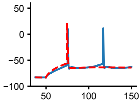
Loss: 115.6153
