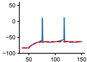
Loss: 117.3634
