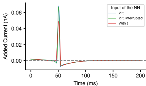
Additional Current Added by the Neural ODE Augmentation
