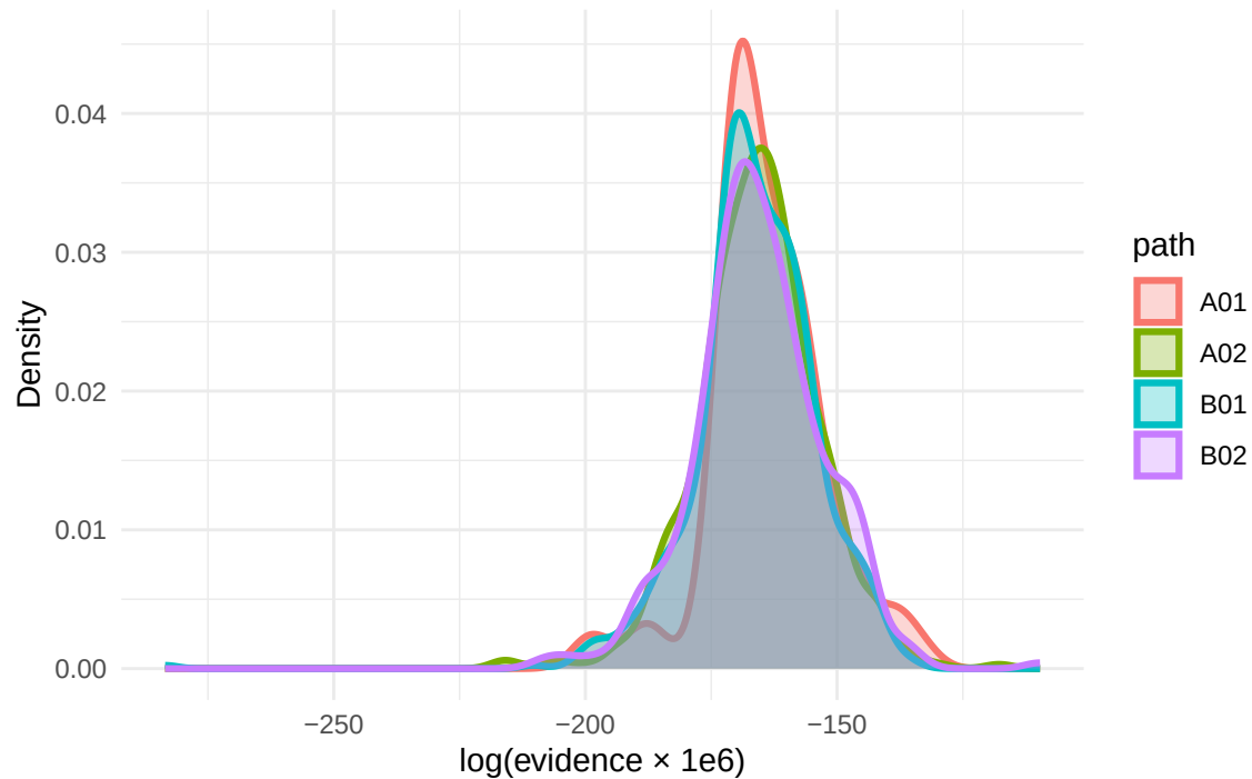
Cluster -1_-2 (rewards: -1,-2 )
