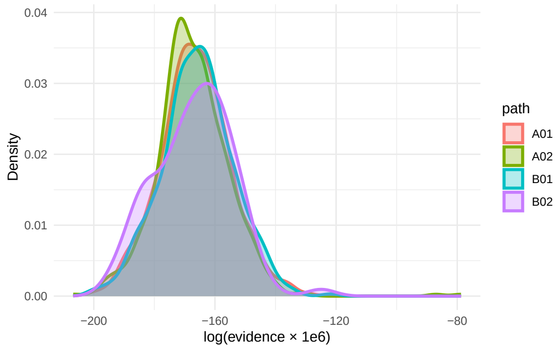
Cluster 1_2 (rewards: 2,1 )
