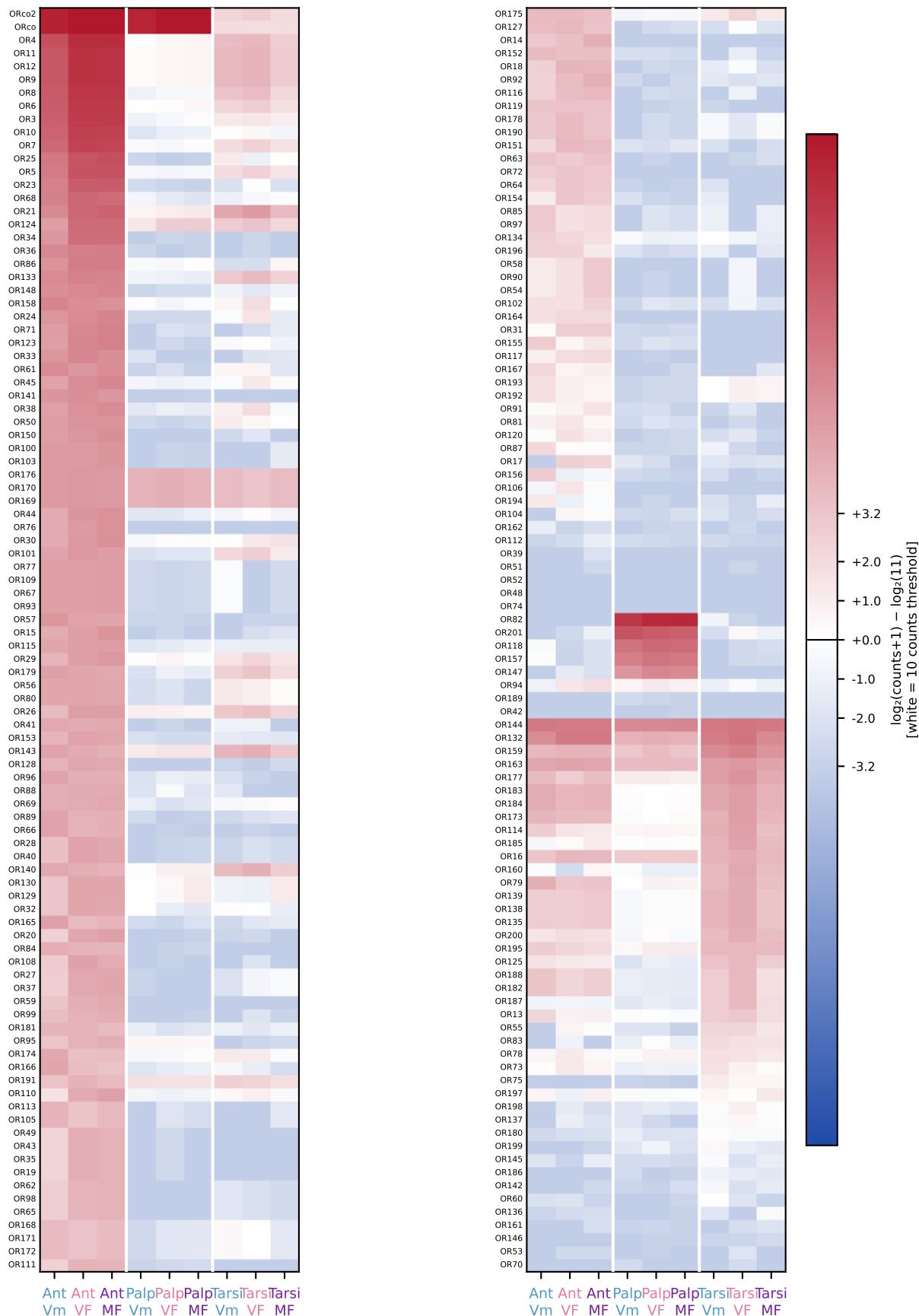
Figure S17 — OR family expression heatmap (n = 192 genes)
