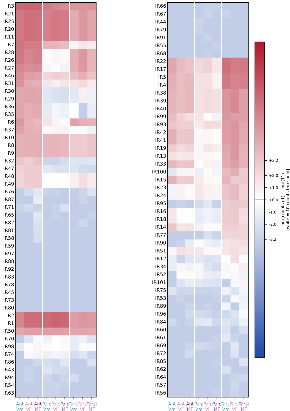
Figure S19 — IR family expression heatmap (n = 101 genes)
