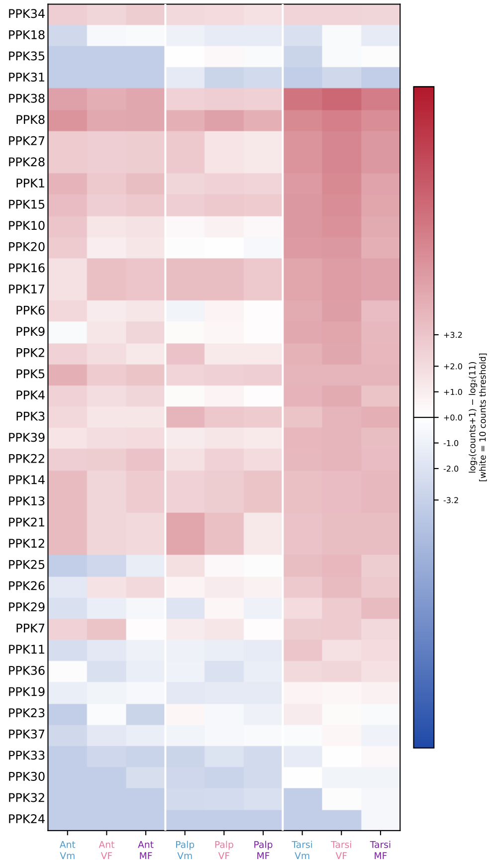
Figure S21 — PPK family expression heatmap (n = 39 genes)
