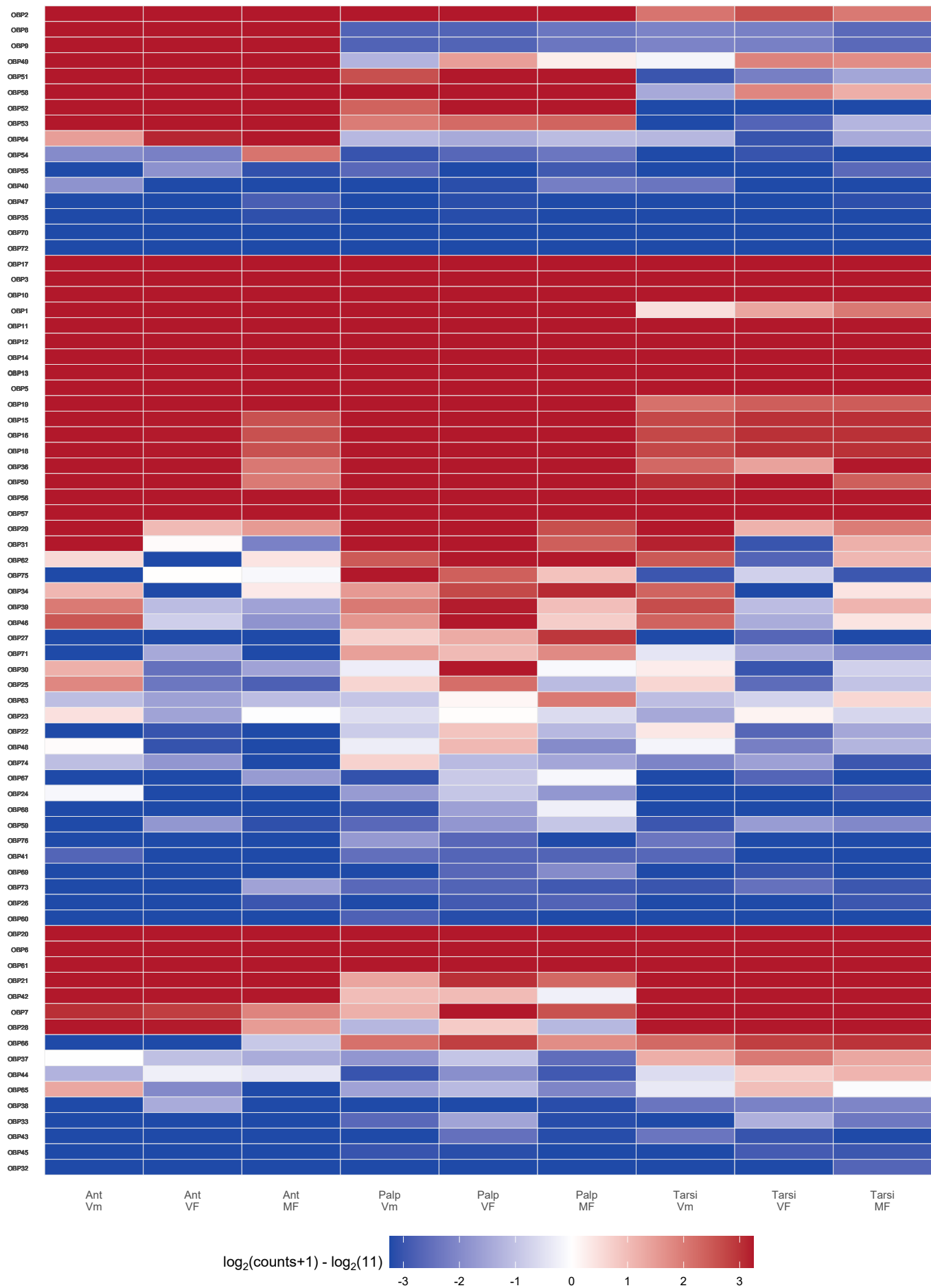
Figure S16. Expression heatmap of the H. illucens odorant-binding protein (OBP) family
