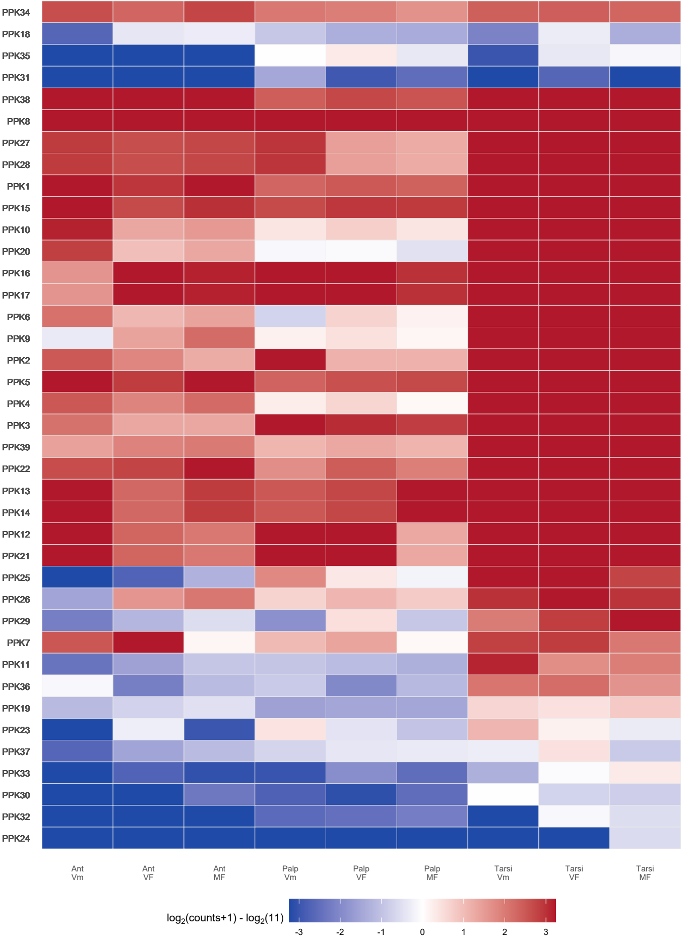
Figure S17. Expression heatmap of the H. illucens pickpocket (PPK) family
