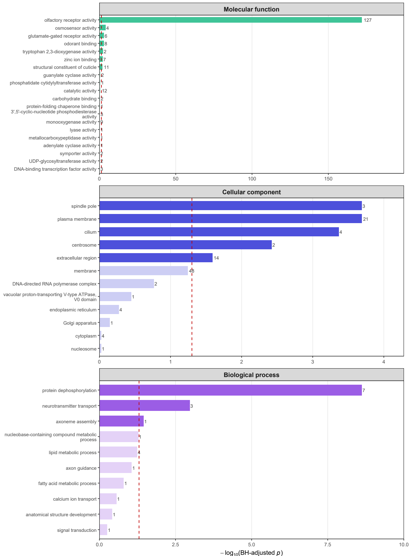
Figure S9. Gene Ontology over-representation among antenna-biased genes
