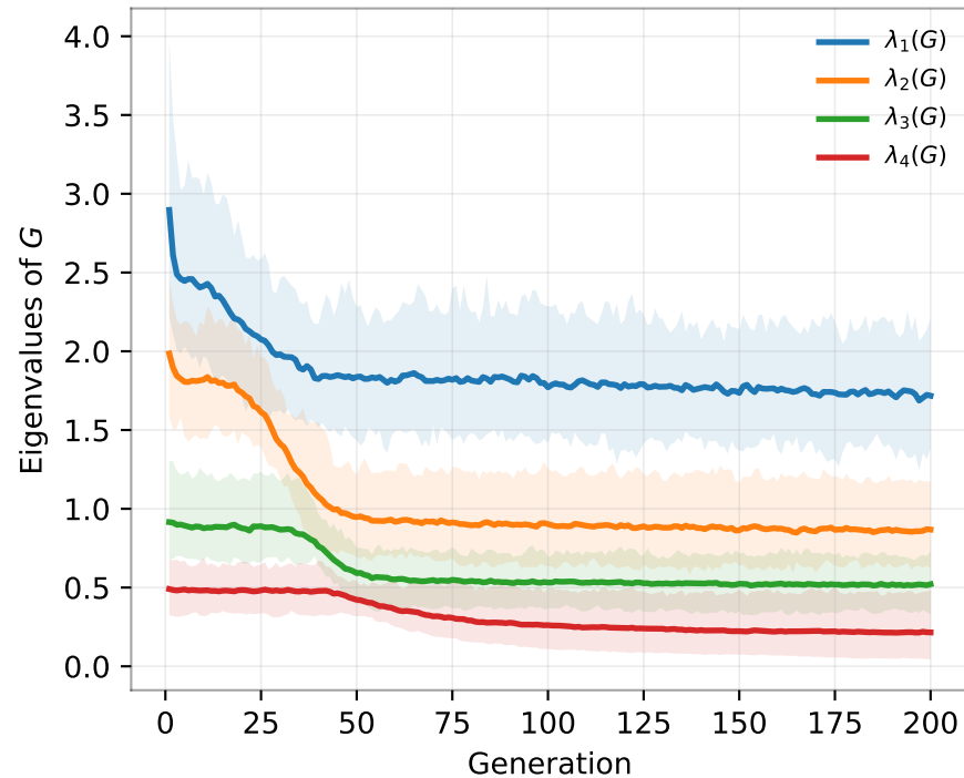
Genetic variance (4 traits, mean \pm 5--95%)
