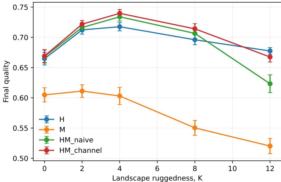
Coupled search on NK landscapes ( D = 4 )
