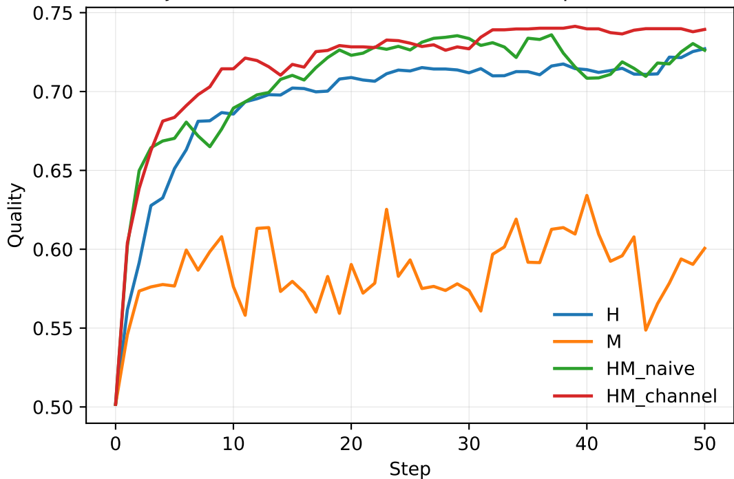
Mean trajectories in an intermediate landscape ( K = 4 , D = 4 )
