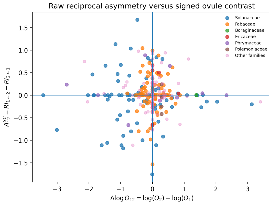
Figure 3: Raw reciprocal asymmetry against signed ovule contrast. The predicted signal is a positive association: points should tend to fall in the upper-right and lower-left quadrants. This figure is a diagnostic, not the final model.
