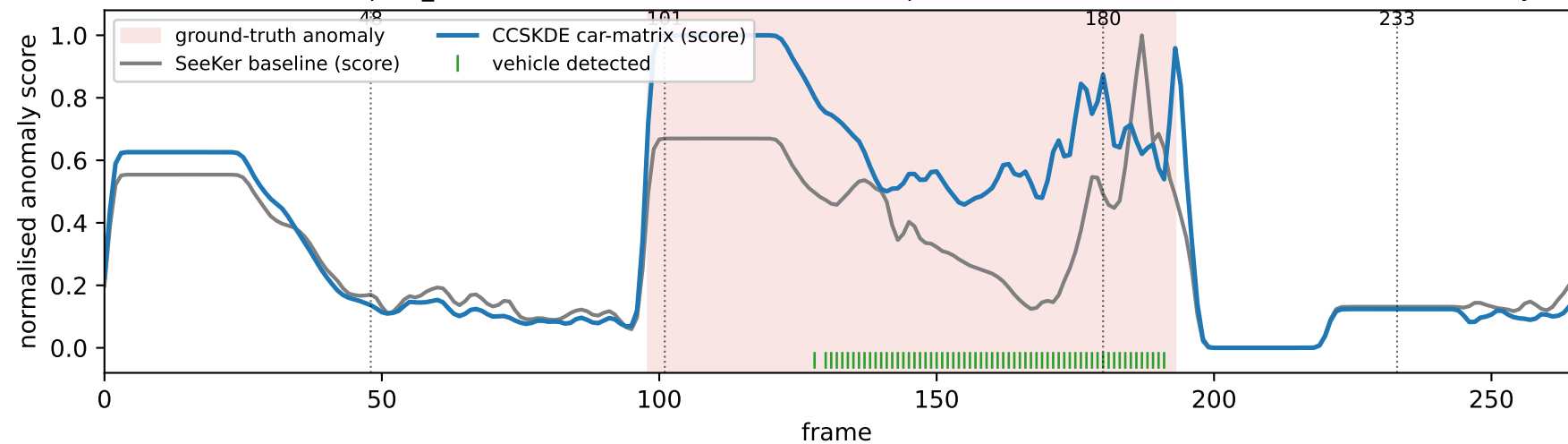
Detection timeline on clip 06_0155: the car-matrix score rises on the pedestrian-vehicle hazard window; the baseline stays low
