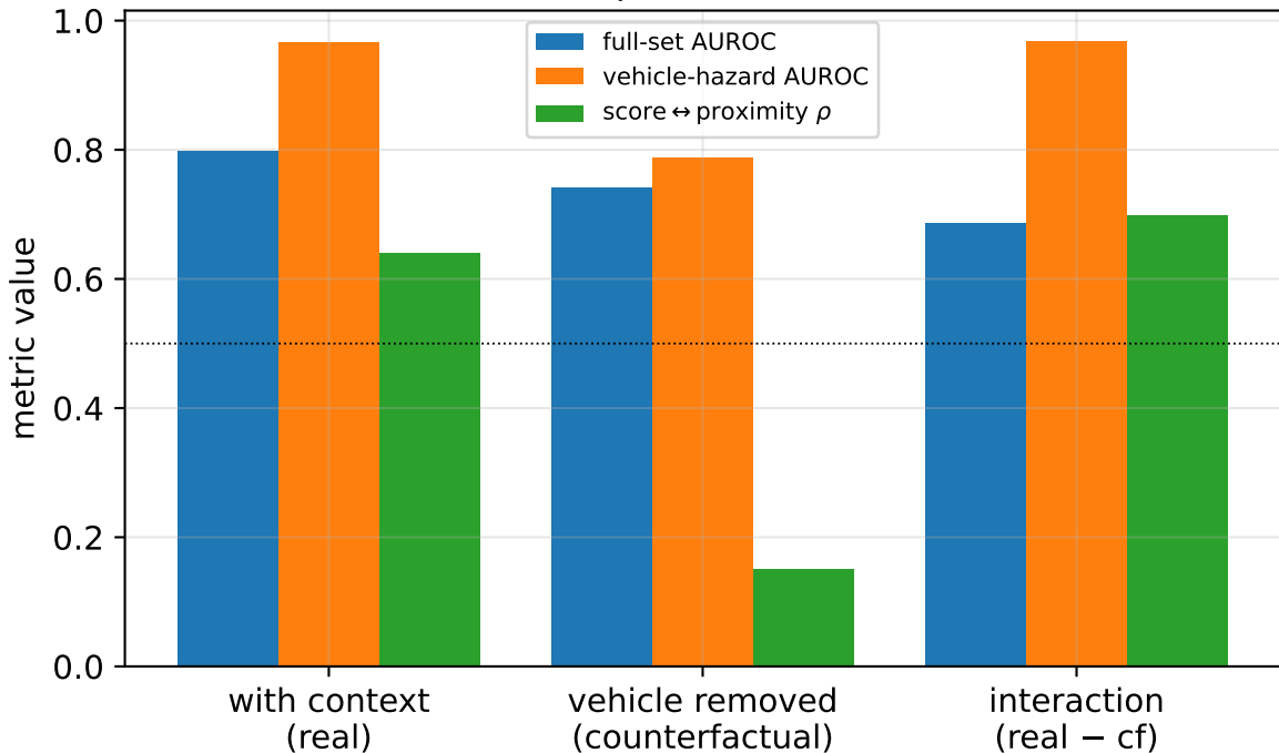
Counterfactual interaction probe (vehicle = car-matrix + FiLM)
