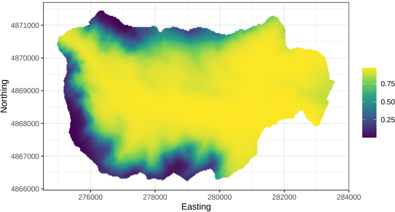
Mean REVI occurrence probability 2018
