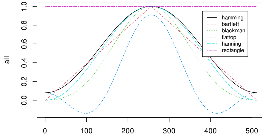
FIGURE 14.3: Different available filters within the seewave package
