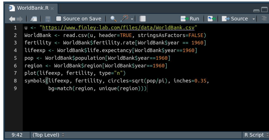
FIGURE 3.1: A script window in RStudio.
