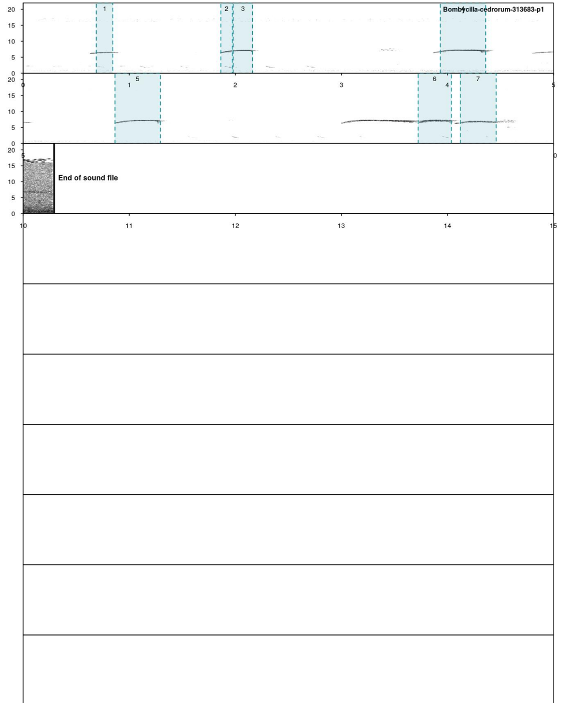
FIGURE 14.6: Spectrogram of identified Cedar Waxwing calls
