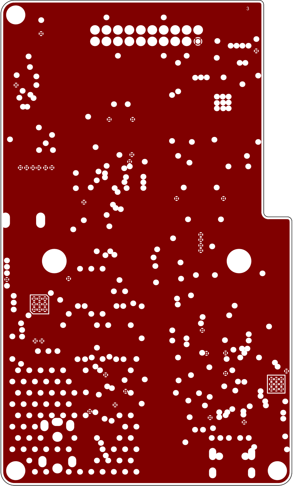
Int2 (PWR) (Scale 2:1)
