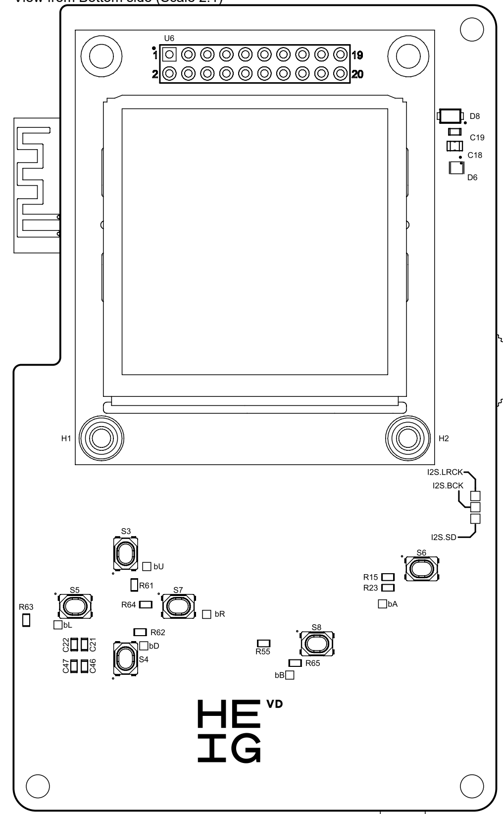
View from Bottom side (Scale 2:1)
