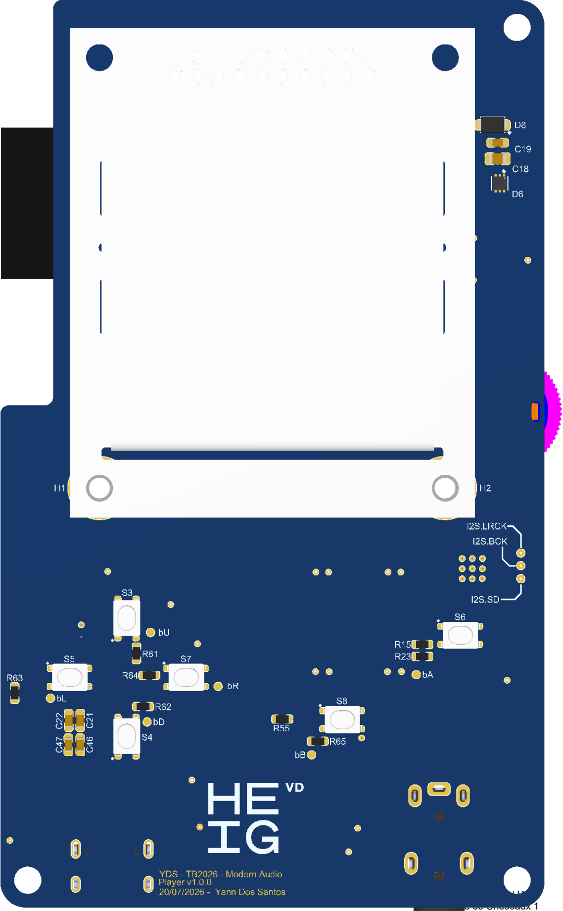
Bottom Realistic View
