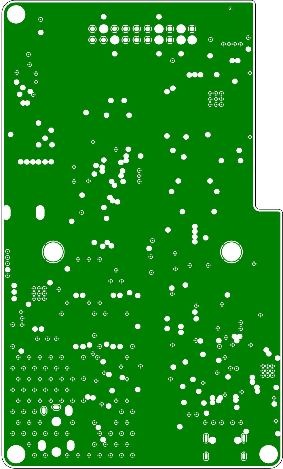
Int1 (GND) (Scale 2:1)
