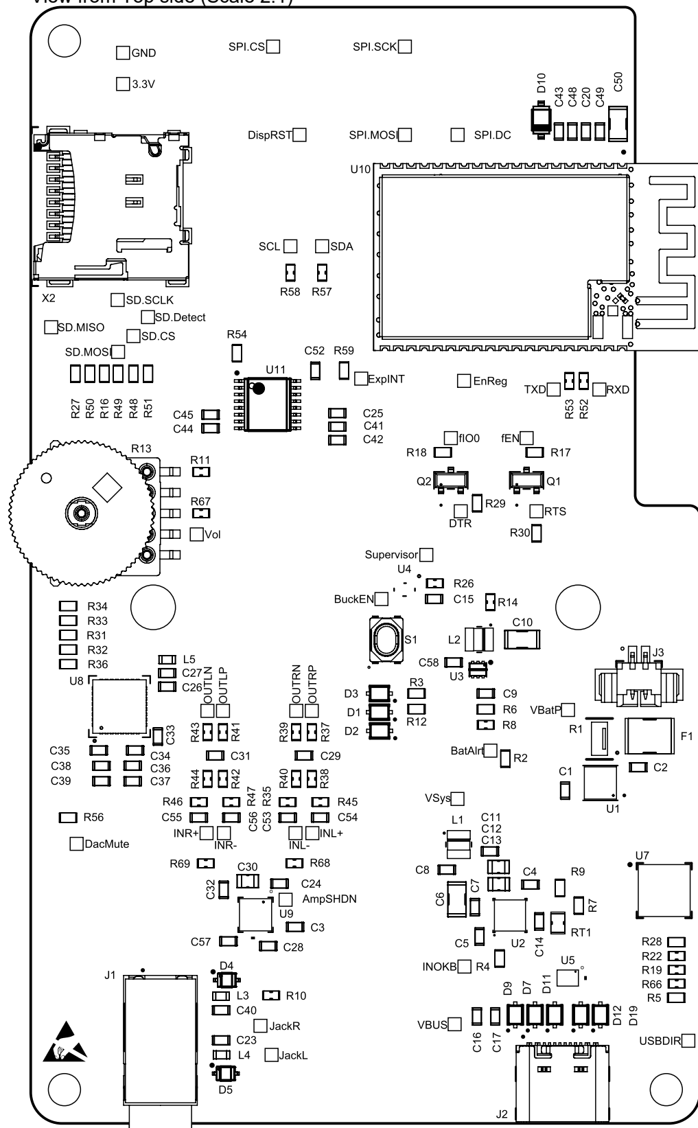
View from Top side (Scale 2:1)
