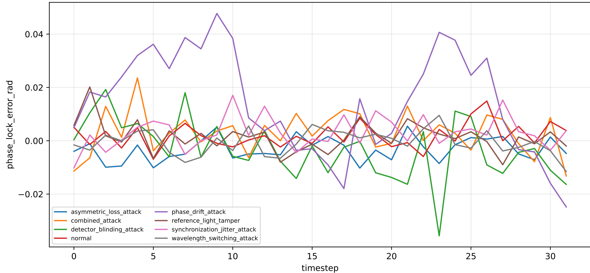
tfqkd_asym: drift over time — phase_lock_error_rad
