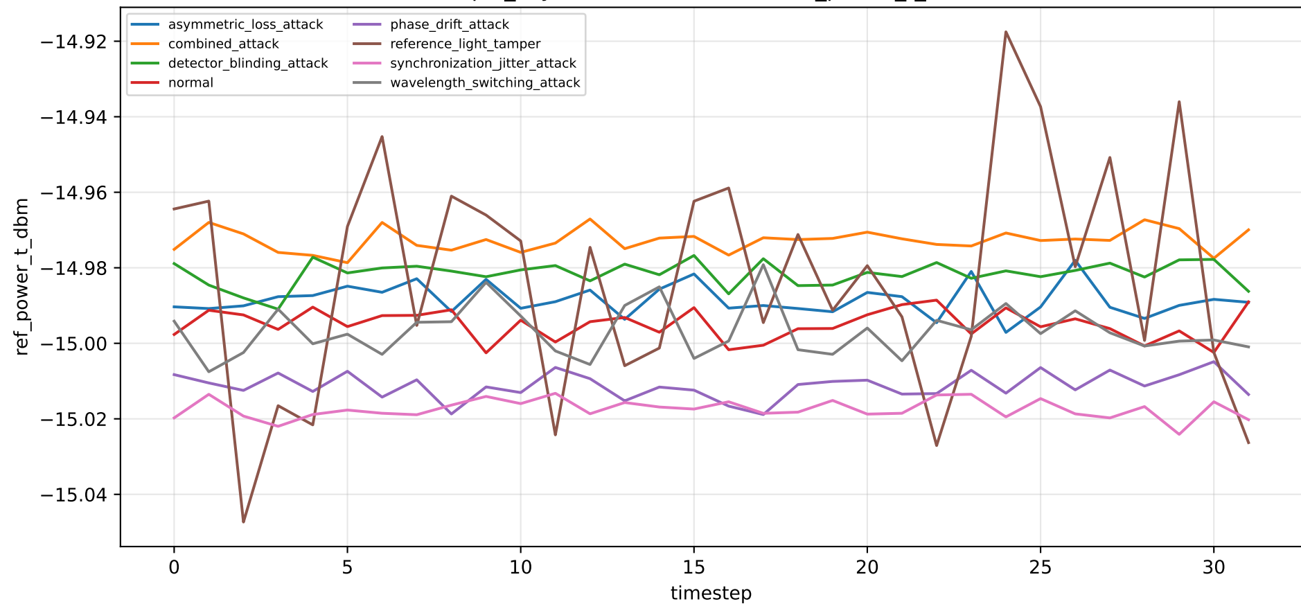
tfqkd_asym: drift over time — ref_power_t_dbm
