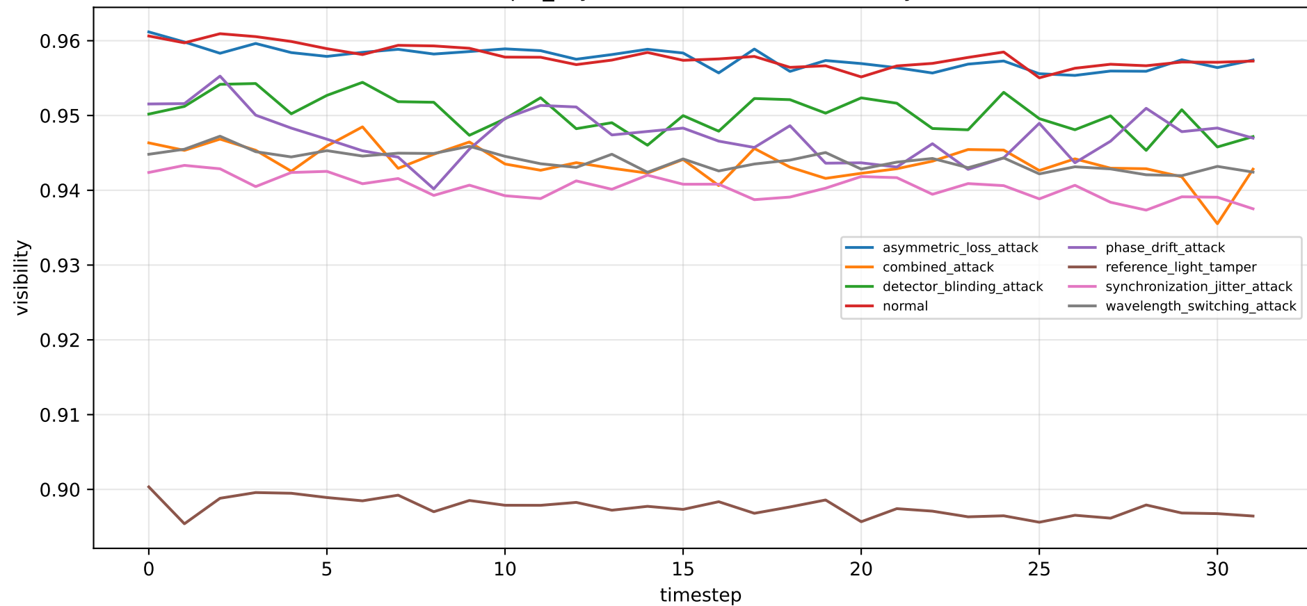
tfqkd_asym: drift over time — visibility
