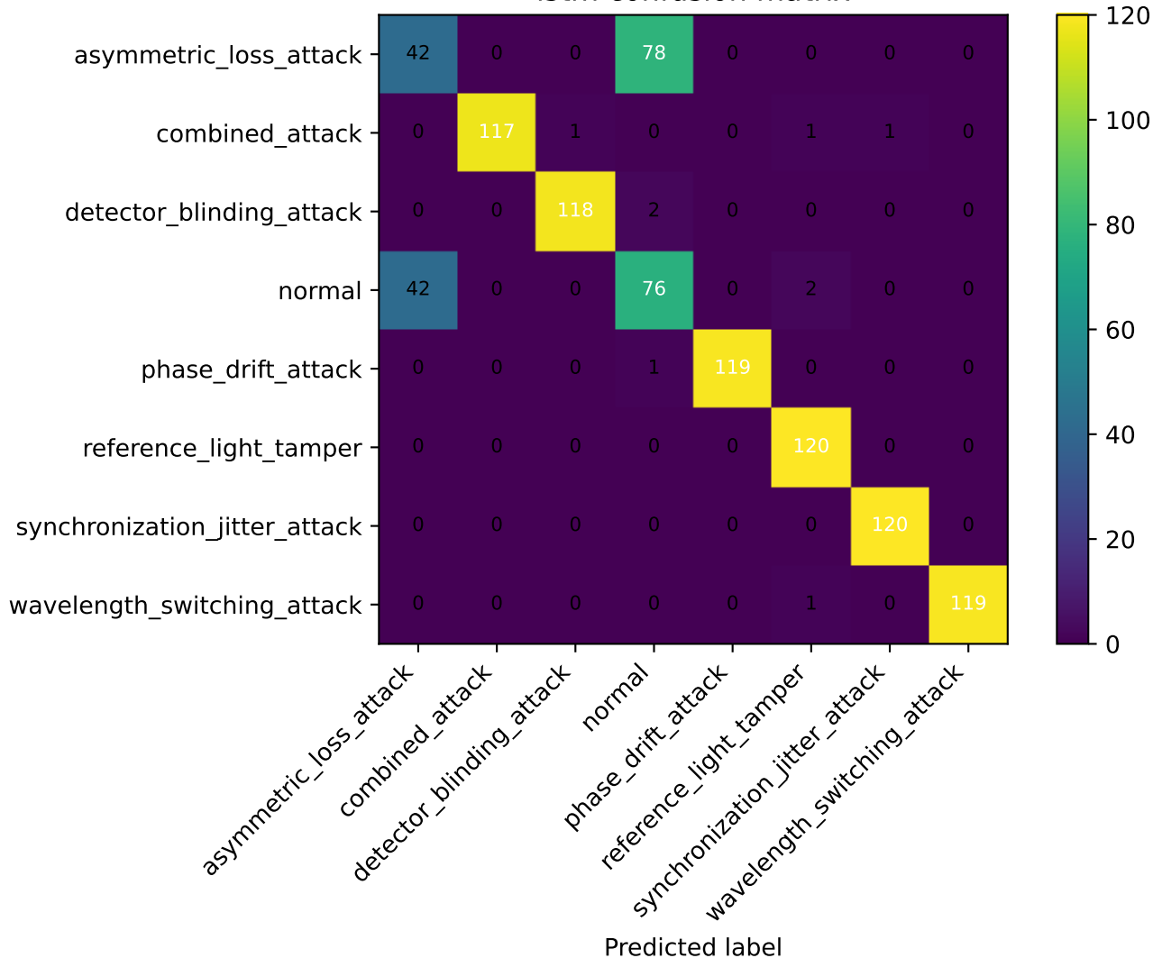
lstm confusion matrix
