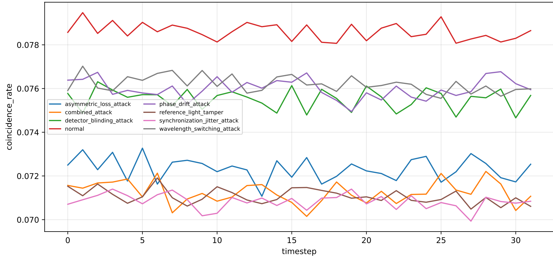
tfqkd_asym: drift over time — coincidence_rate
