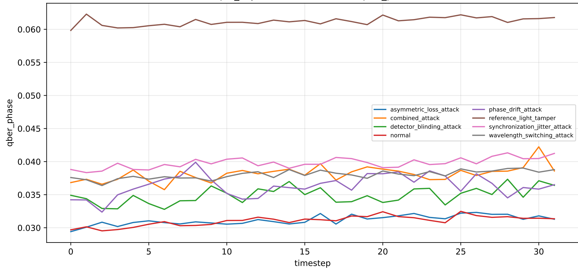
tfqkd_asym: drift over time — qber_phase
