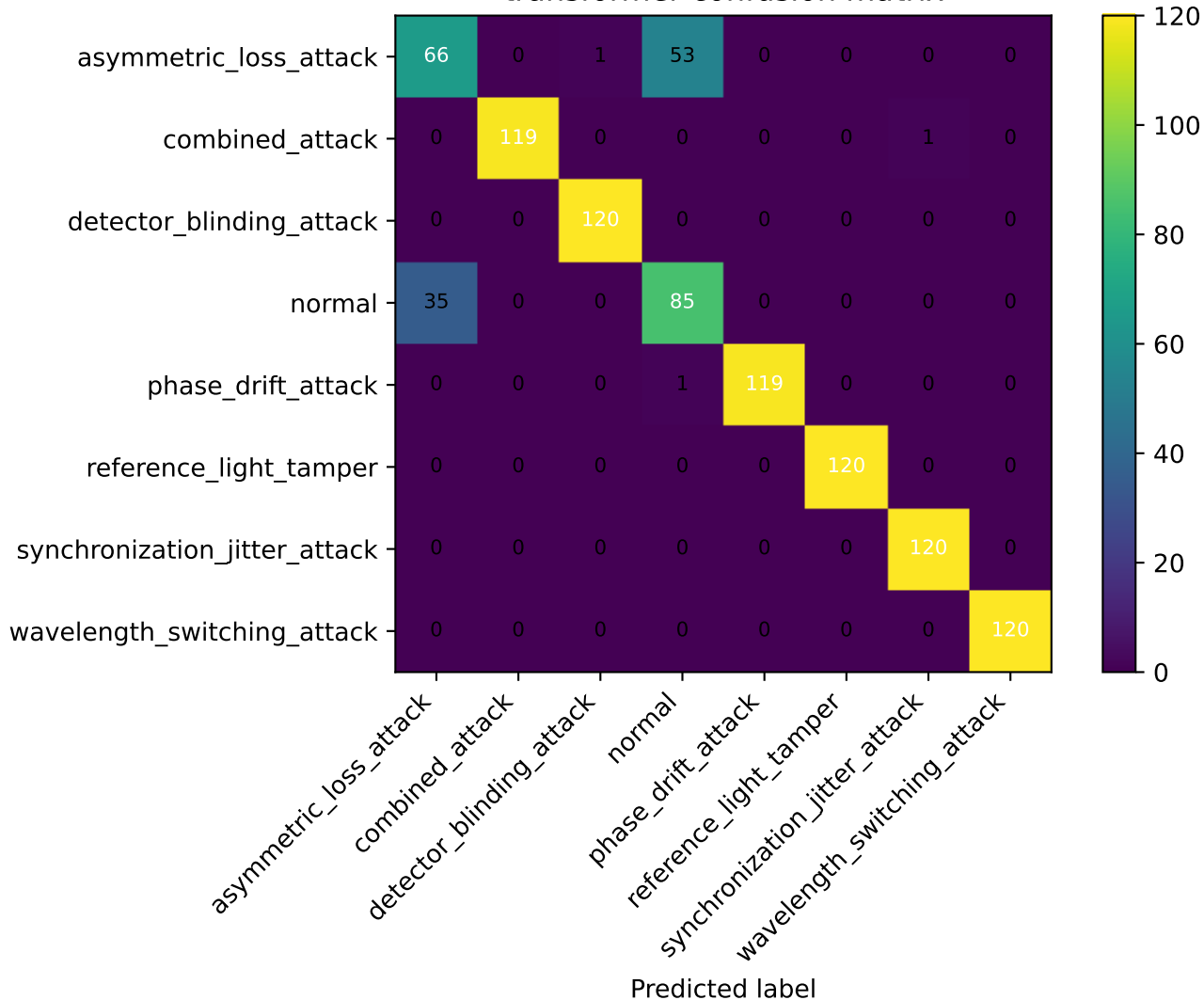
transformer confusion matrix
